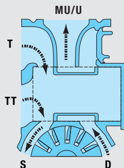
PUMPED DELIVERY From tank or trailer
