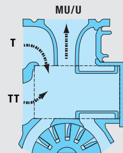
GRAVITY DISCHARGE From tank or trailer
