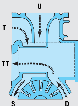
SELF-LOADING From trailer or external tank
